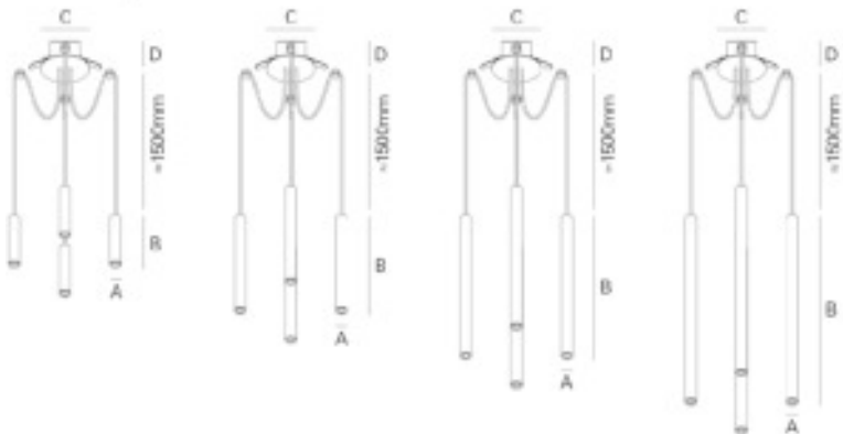
Recessed ceiling rose version
